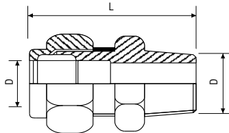
Unión universal bicónica L = 35 mm D = 14 mm A = 3/8"
