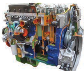
Sectioned engine Mercedes atego, PLD system (injection pump) complete with all parts
