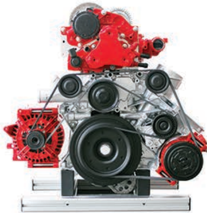
Diesel DOHC Common Rail engine 1/2 cutaway model
