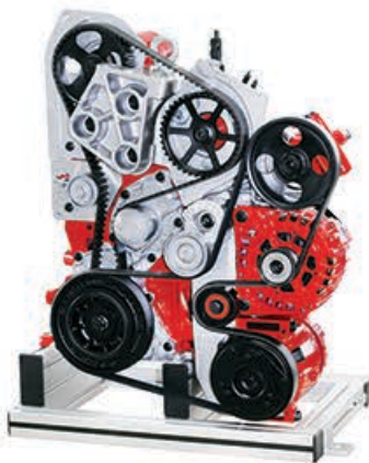
Diesel OHC Common Rail Engine 1/2 cutaway model
