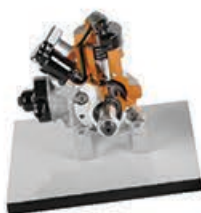
CP4 Bosch high pressure pump Cutaway model
