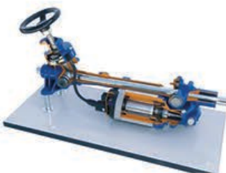
Electrical rack and pinion steering Cutaway model
