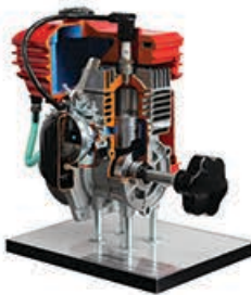
2 stroke petrol engine Cutaway model
