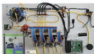
LPG TIMED SEQUENTIAL INJECTION FOR ELECTRONIC INJECTION ENGINES (wall-mounted) – cutaway training model
