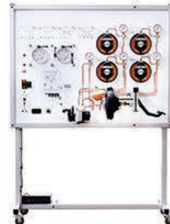
Anti-Lock Braking system BOSCH ABS 5.3 training stand
